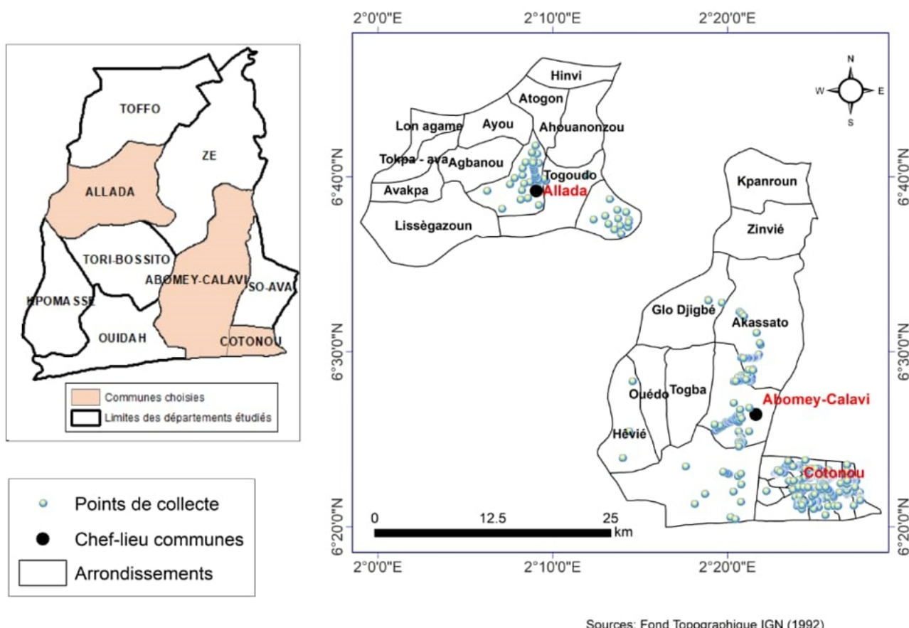
Figure 1: Map of the study area (SEHOUN et al. (2021))
